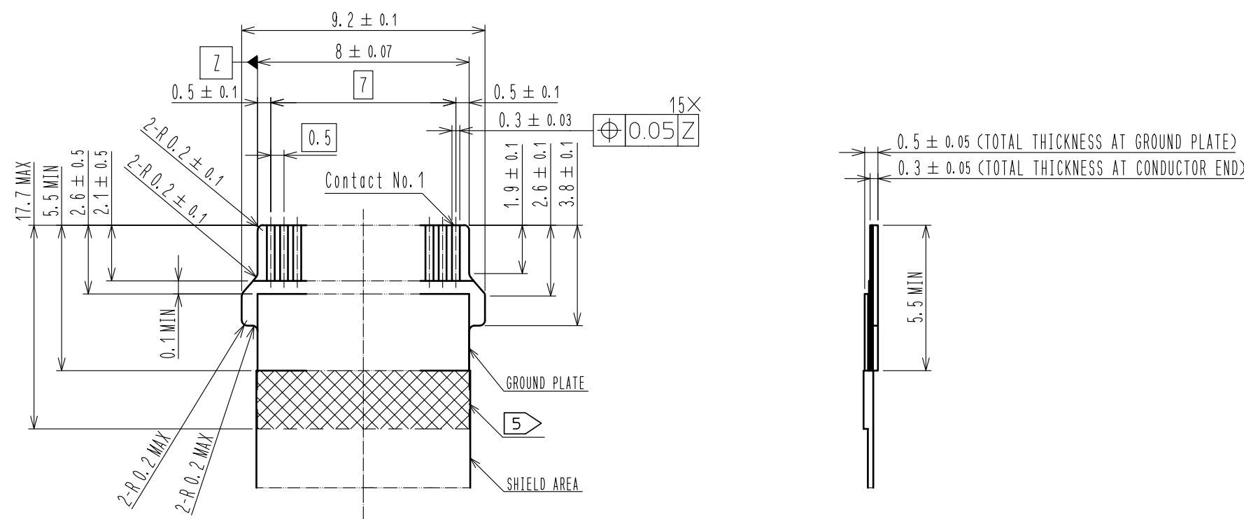
FFC CONFIGURATION (REFERENCE EXAMPLE) (SCALE:FREE)
